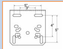
UBG-500 Mounting Plate UBG-500F Mounting Plate
