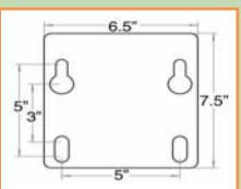
GBA-180 Mounting Plate
