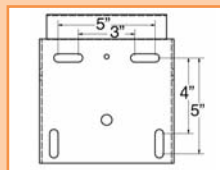
GBA-648 Mounting Plate GBA-548 Mounting Plate
