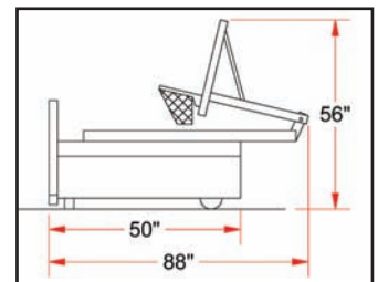
PBB-200 folded dimensions
