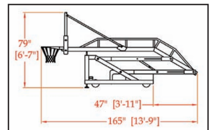
PBEL96 folded dimensions
