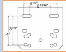
G-35 Mounting Plate
