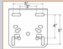
GBSG-50 Mounting Plate
