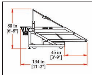
PBEL66 folded dimensions
