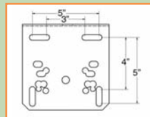
GDR-54 Mounting Plate
