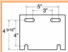
GBA-642 Mounting Plate GBA-542 Mounting Plate
