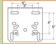
GB-55 Mounting Plate
