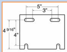
GBA-342A Mounting Plate GBA-600 Mounting Plate
