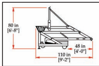
PBEL54 folded dimensions
